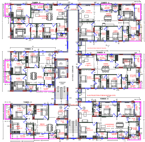
Building plan
