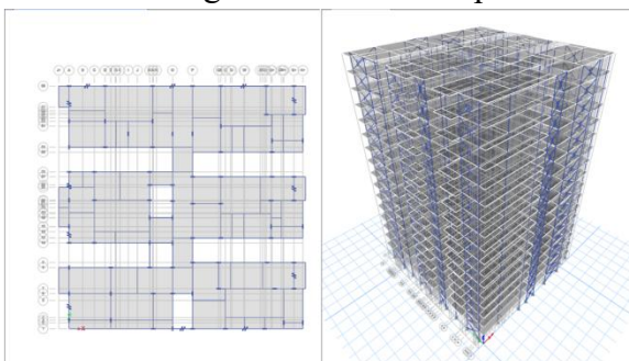
Building with viscous dampers
