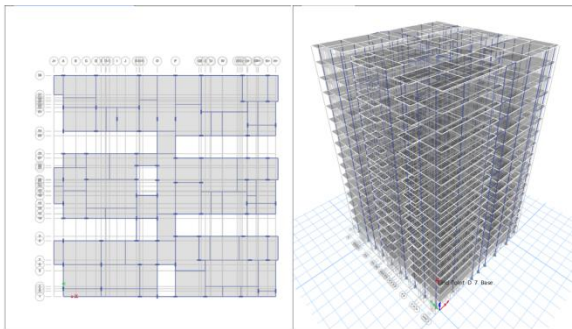
Building model without dampers
